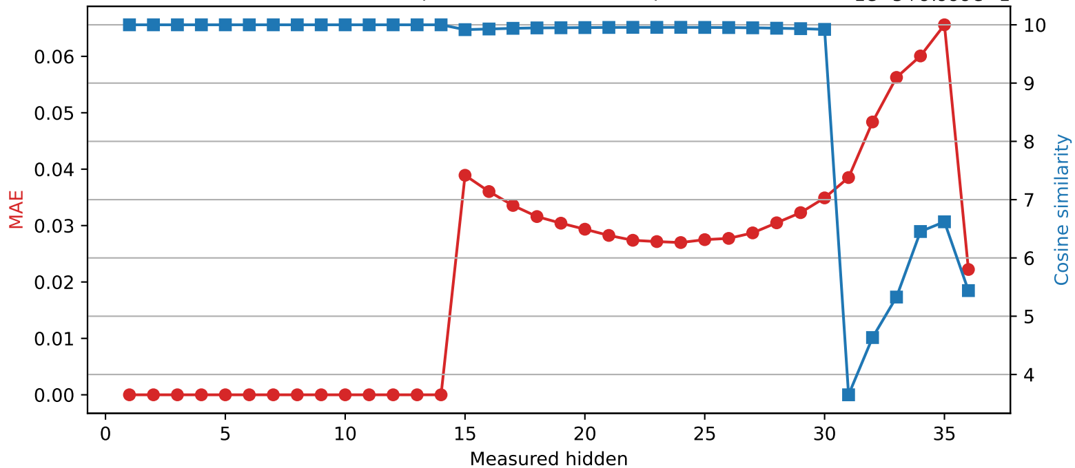
Qwen2.5-3B | Quantized layer 14 | float16 → int8
