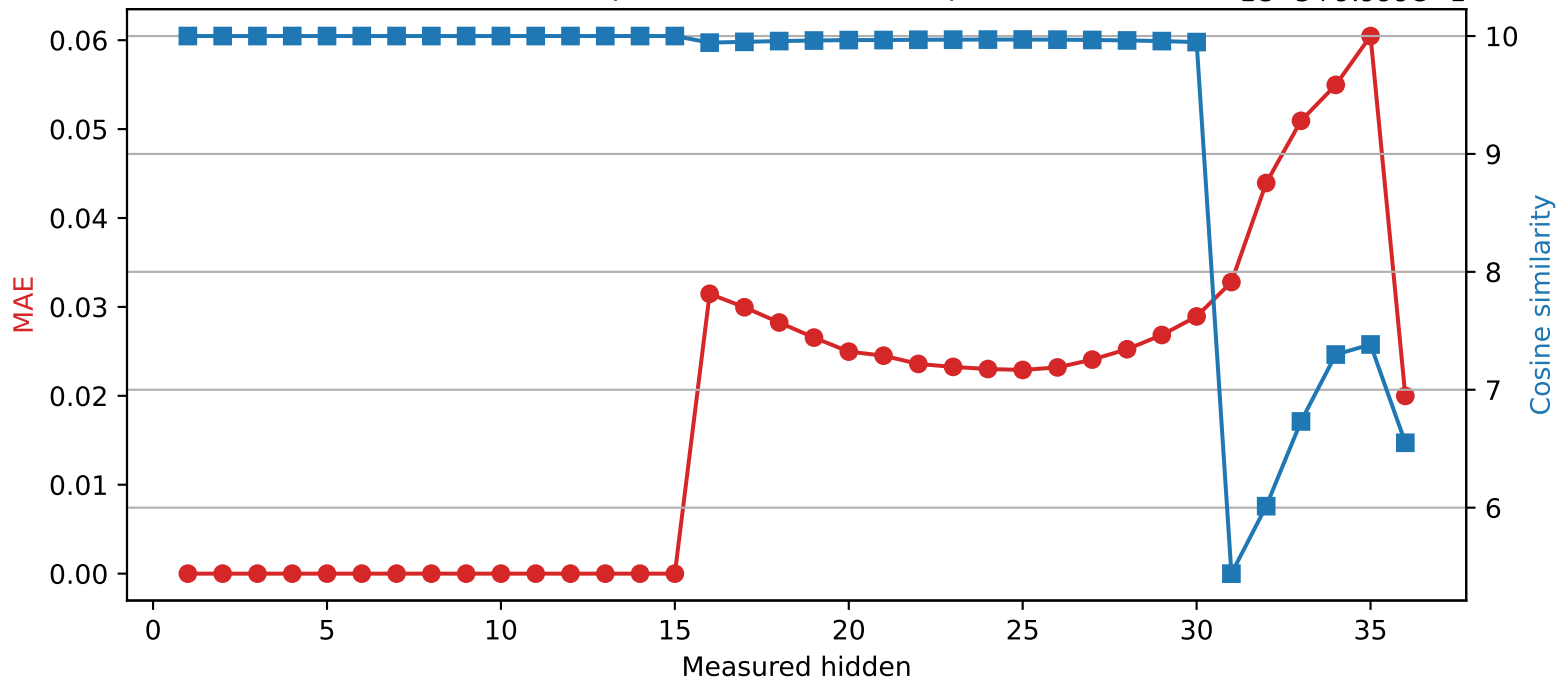
Qwen2.5-3B | Quantized layer 15 | float16 → int8
