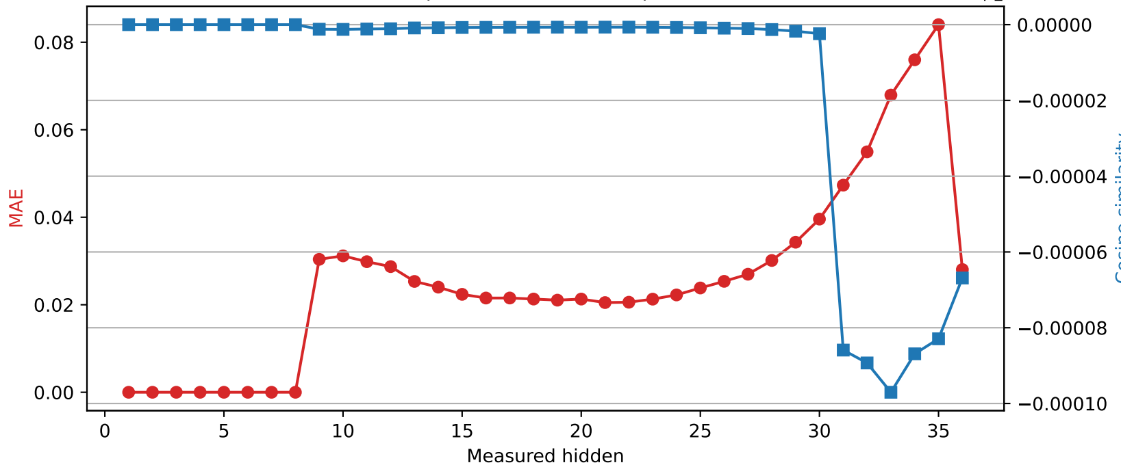
Qwen2.5-3B | Quantized layer 8 | float16 → int8
