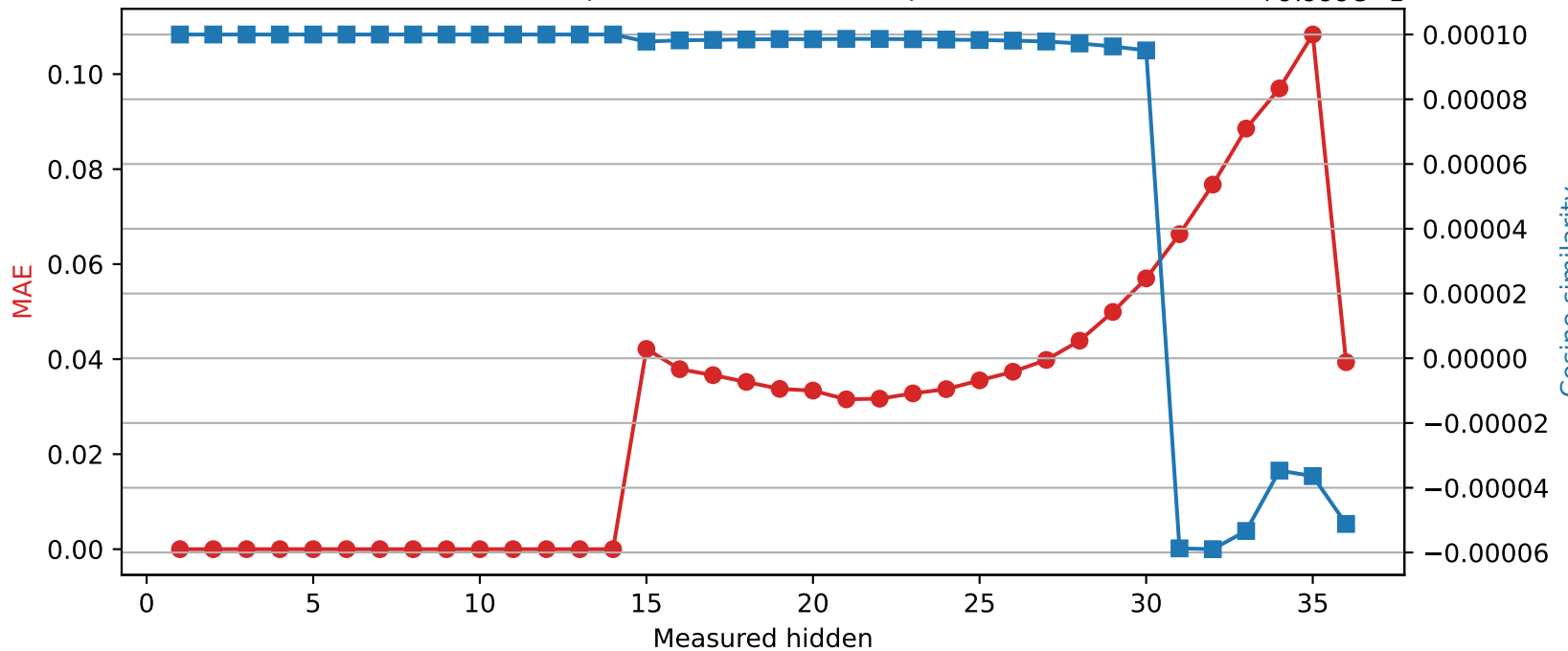
Qwen2.5-3B | Quantized layer 14 | float16 → int8
