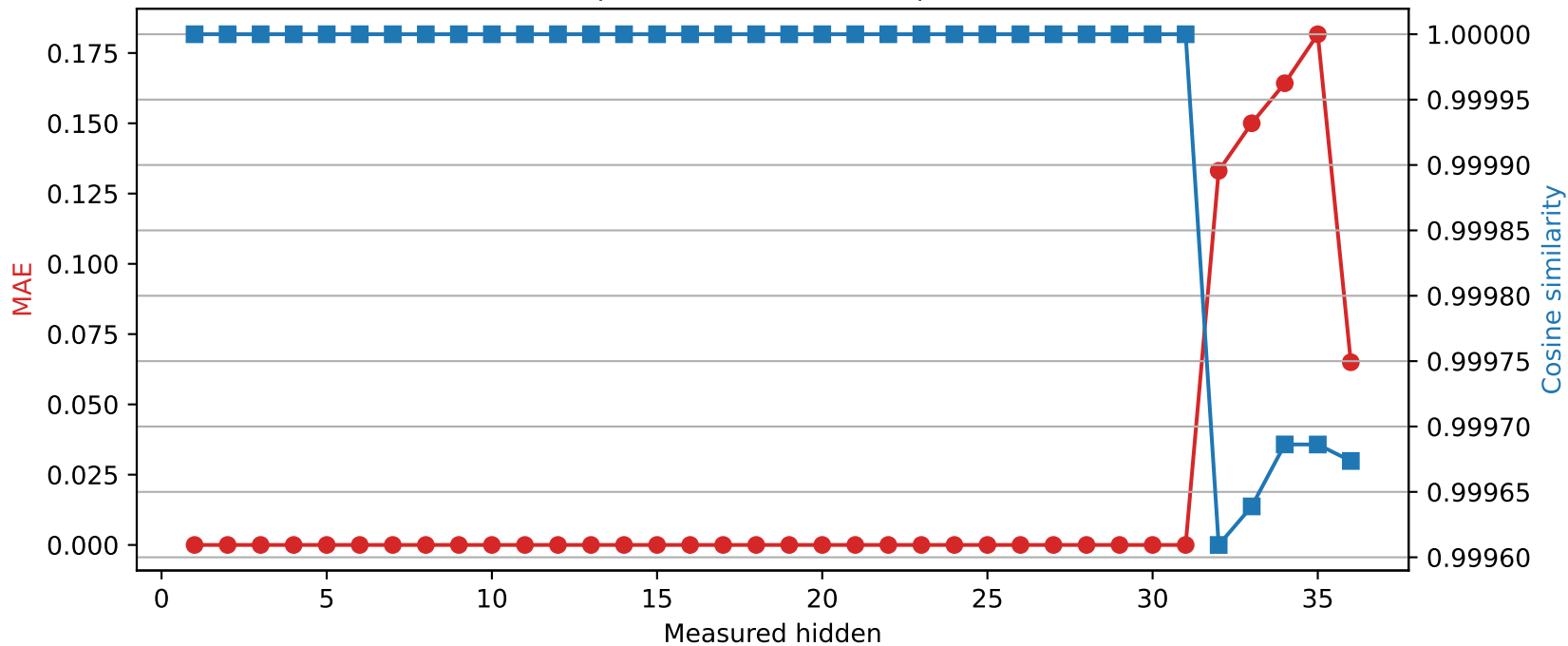
Qwen2.5-3B | Quantized layer 31 | float16 → int8
