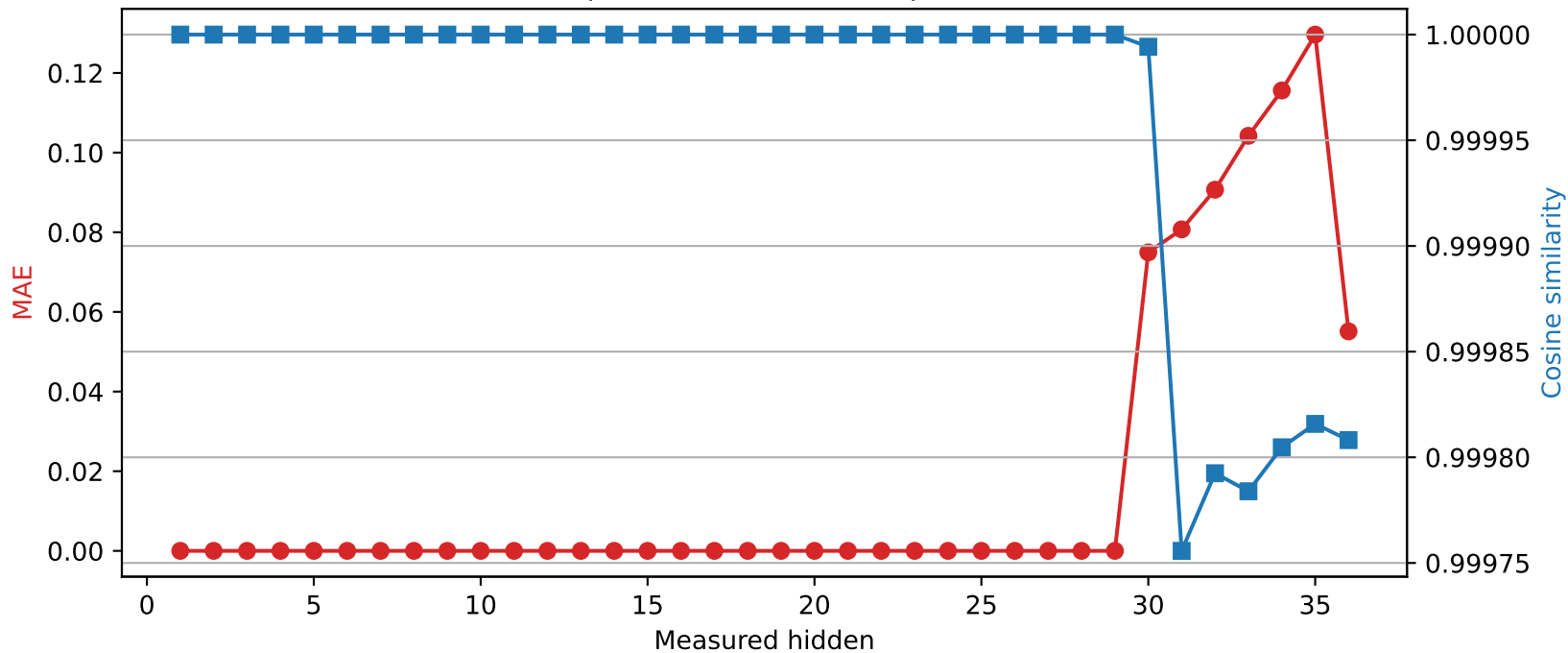
Qwen2.5-3B | Quantized layer 29 | float16 → int8
