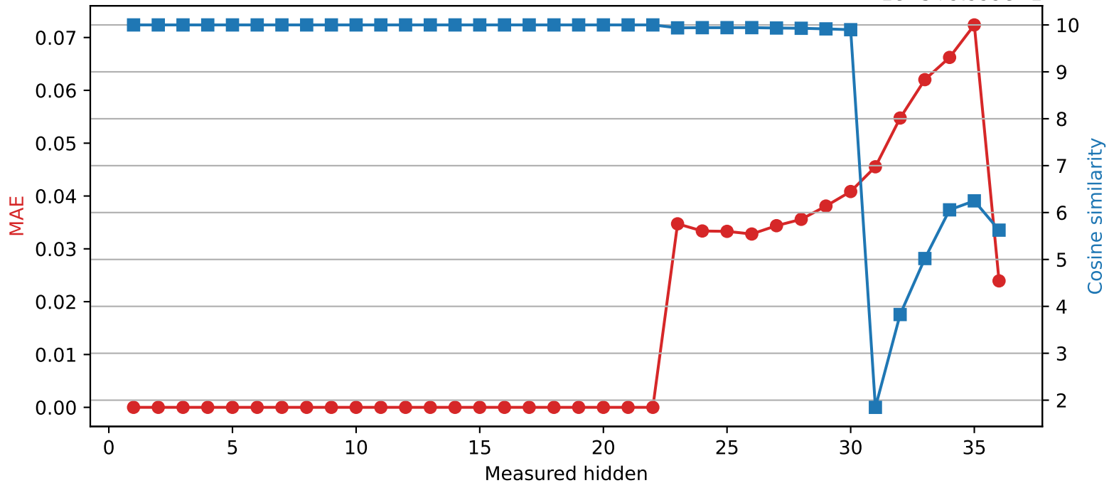
Qwen2.5-3B | Quantized layer 22 | float32 → int8
