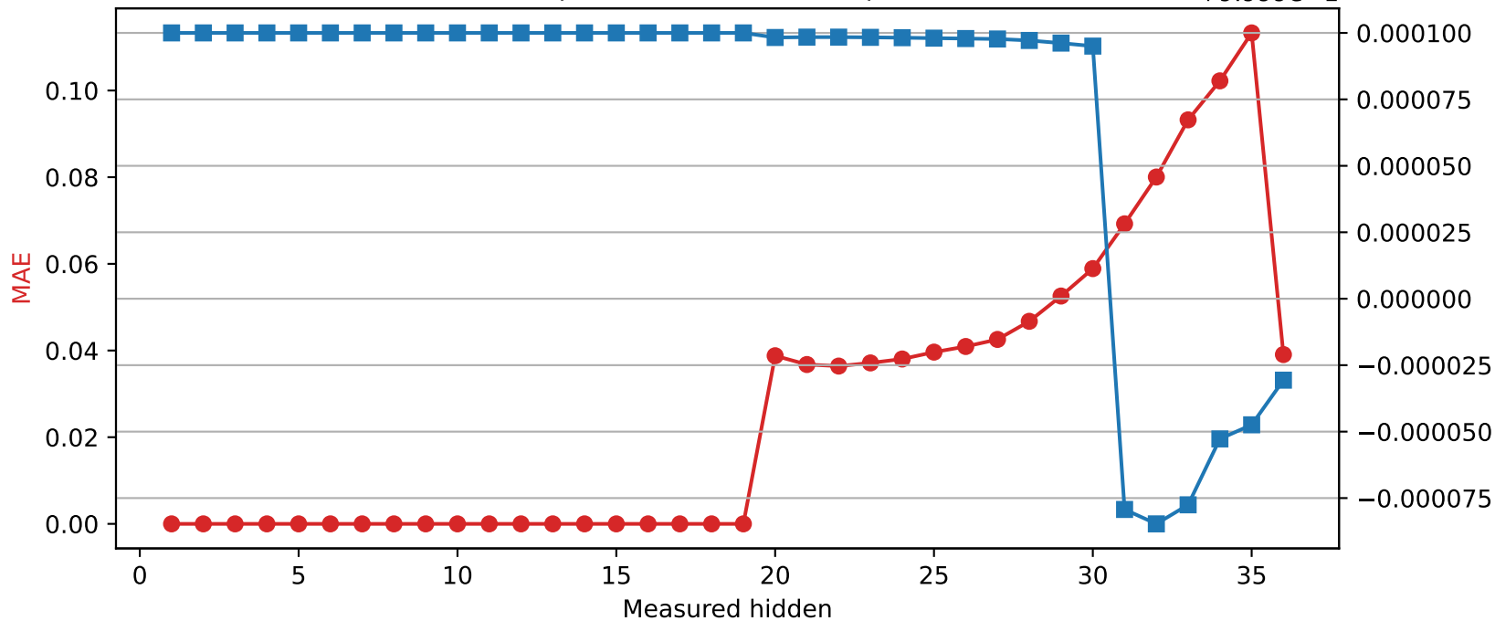
Qwen2.5-3B | Quantized layer 19 | float32 → int8
