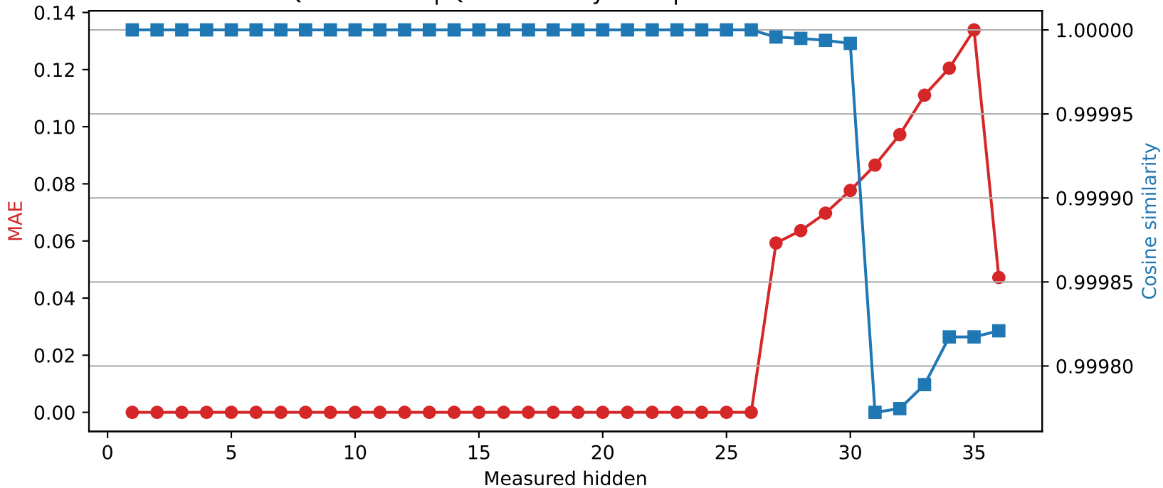
Qwen2.5-3B | Quantized layer 26 | float32 → int8
