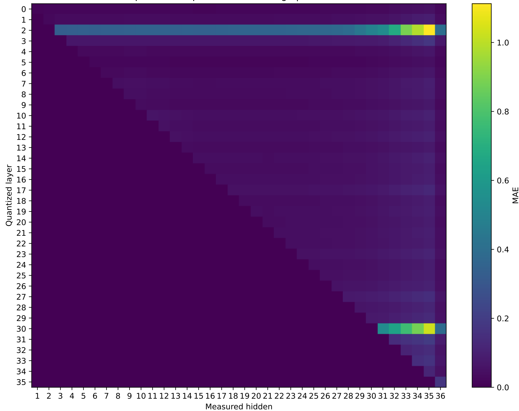
Qwen2.5-3B Prompt 2: MAE representation damage | float32 \rightarrow int8
