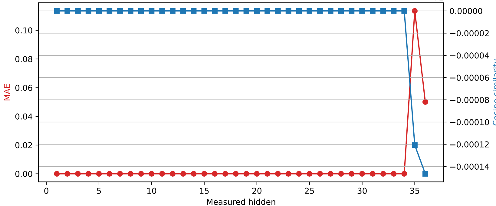
Qwen2.5-3B | Quantized layer 34 | float32 → int8
