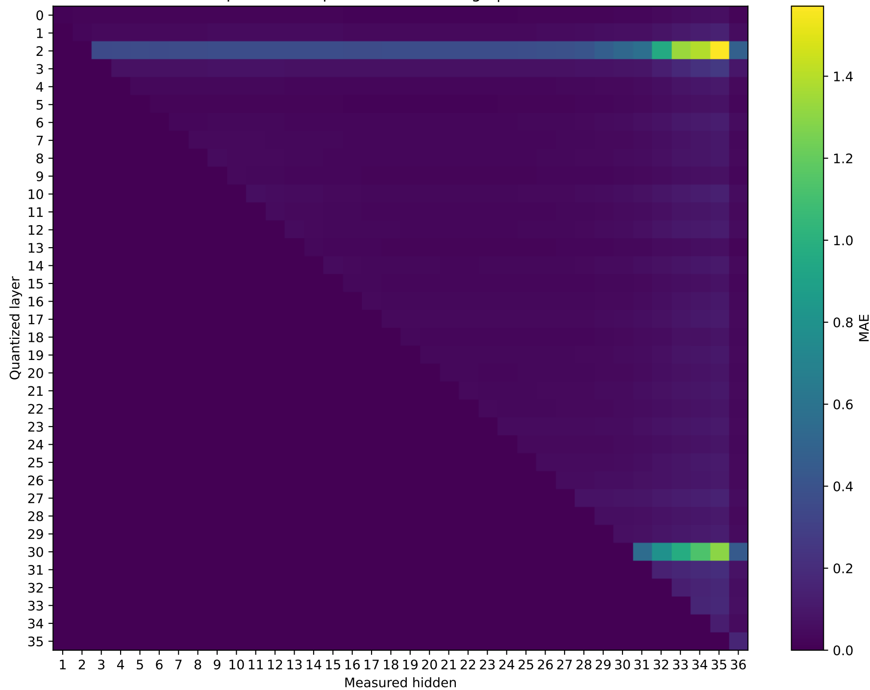
Qwen2.5-3B Prompt 3: MAE representation damage | float32 → int8
