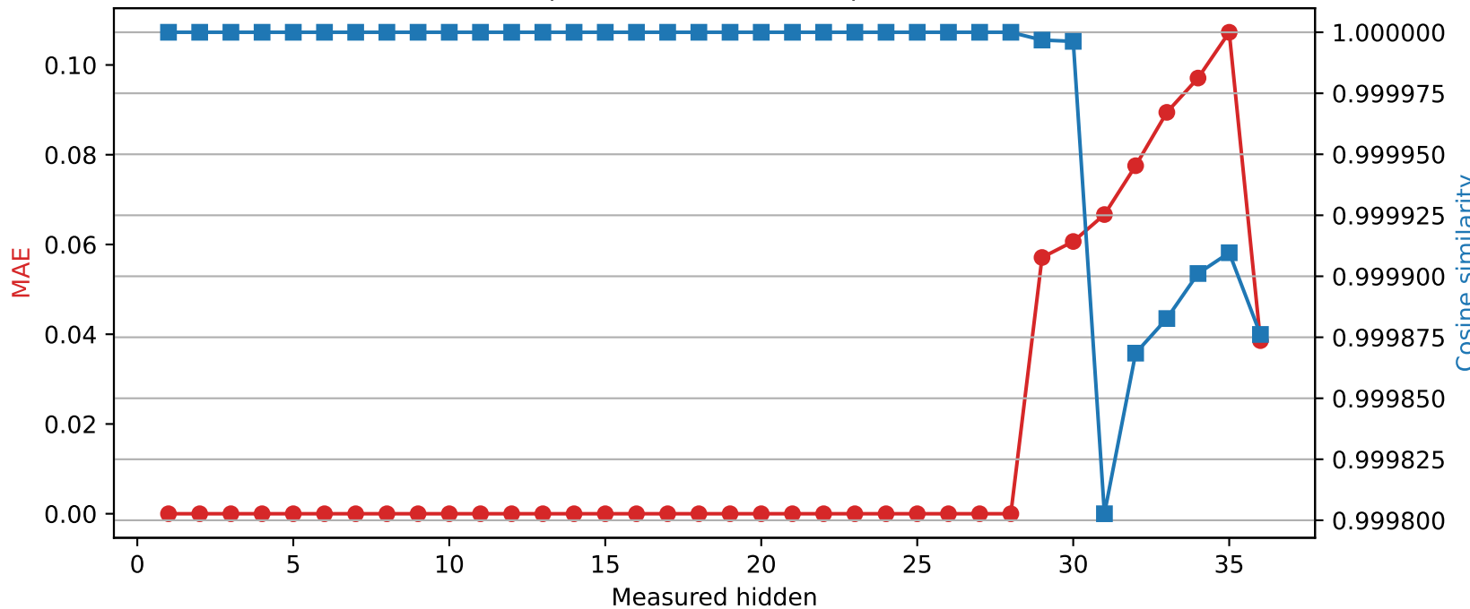
Qwen2.5-3B | Quantized layer 28 | float32 → int8
