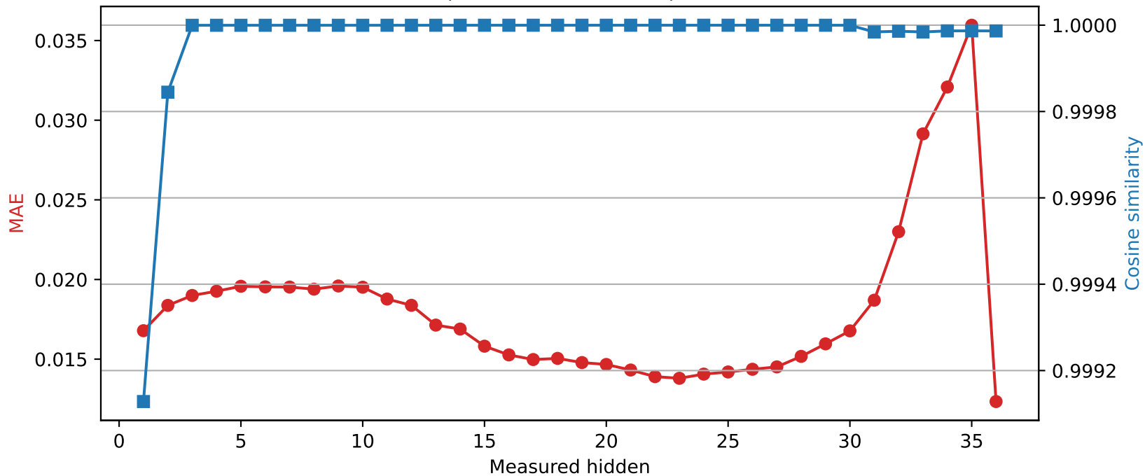
Qwen2.5-3B | Quantized layer 0 | float32 → int8
