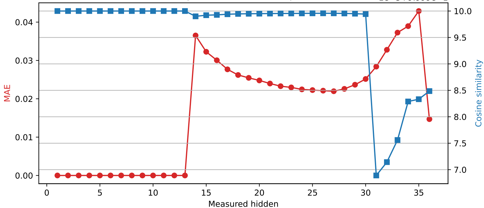
Qwen2.5-3B | Quantized layer 13 | float32 → int8
