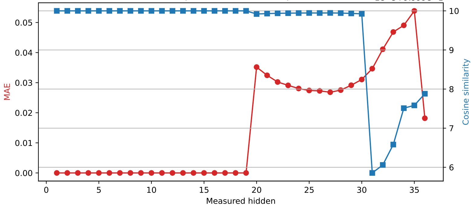
Qwen2.5-3B | Quantized layer 19 | float32 → int8
