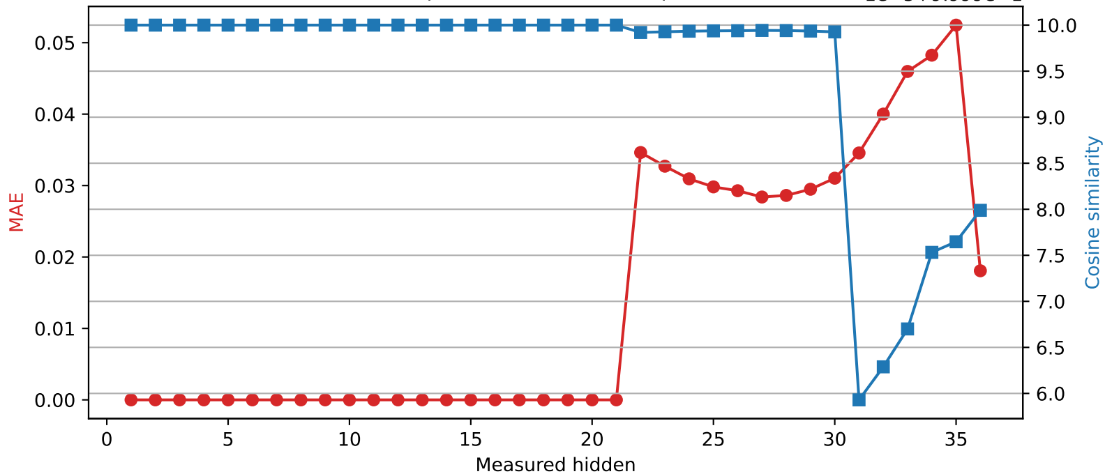
Qwen2.5-3B | Quantized layer 21 | float32 → int8
