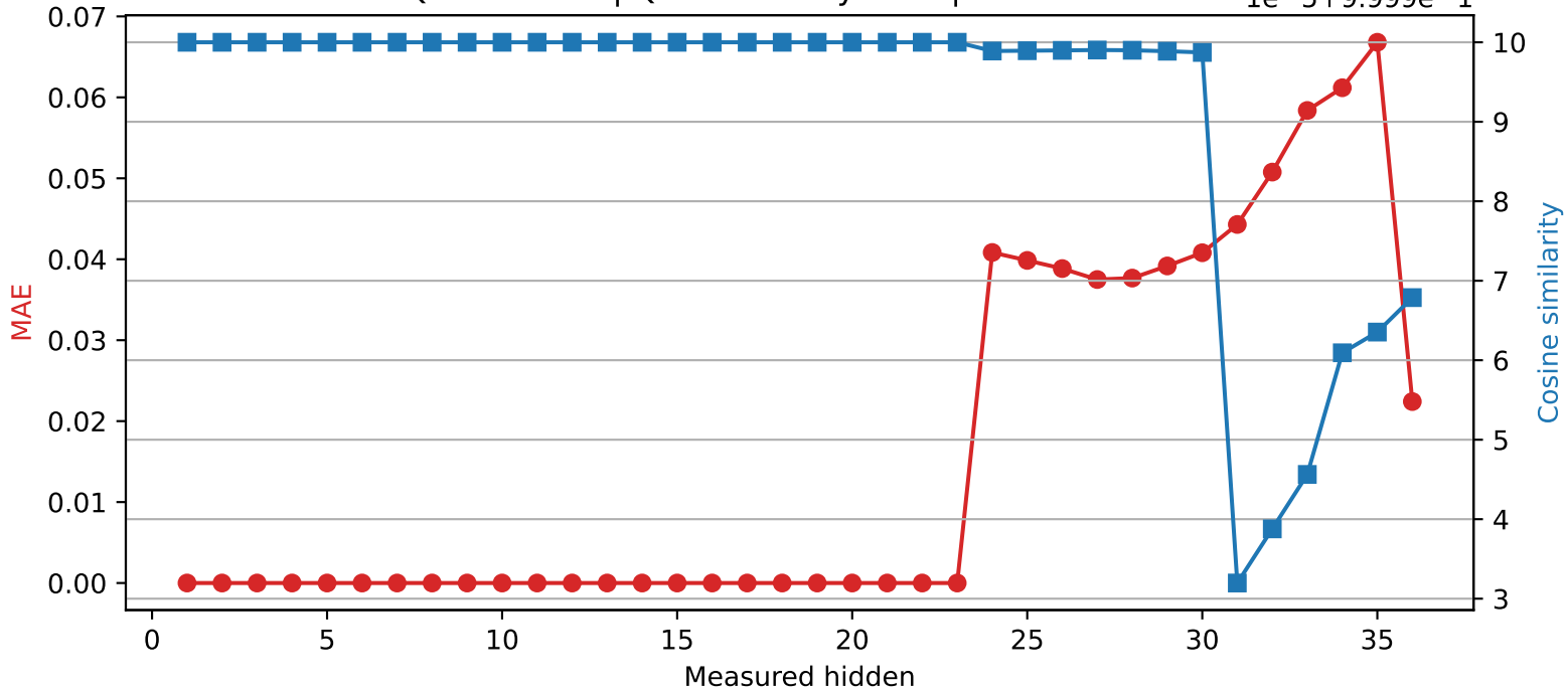
Qwen2.5-3B | Quantized layer 23 | float32 → int8
