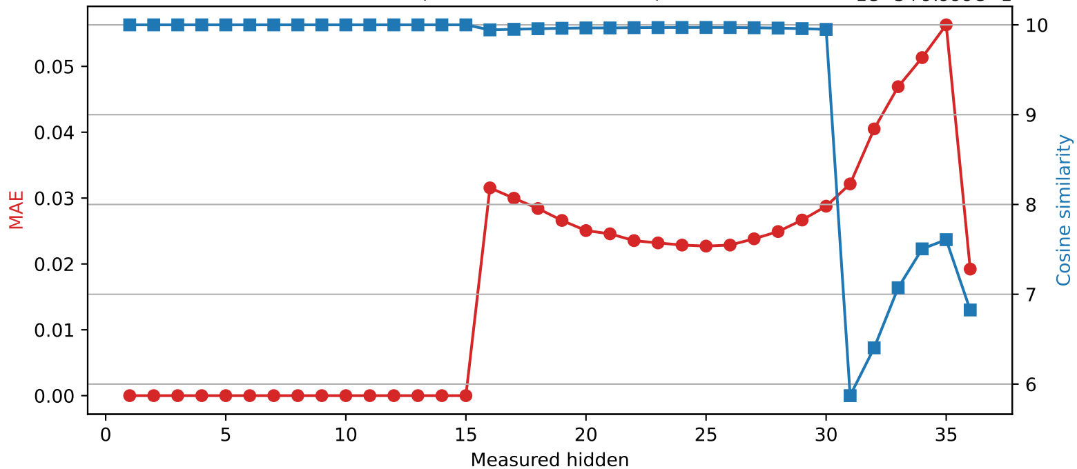
Qwen2.5-3B | Quantized layer 15 | float64 → int8
