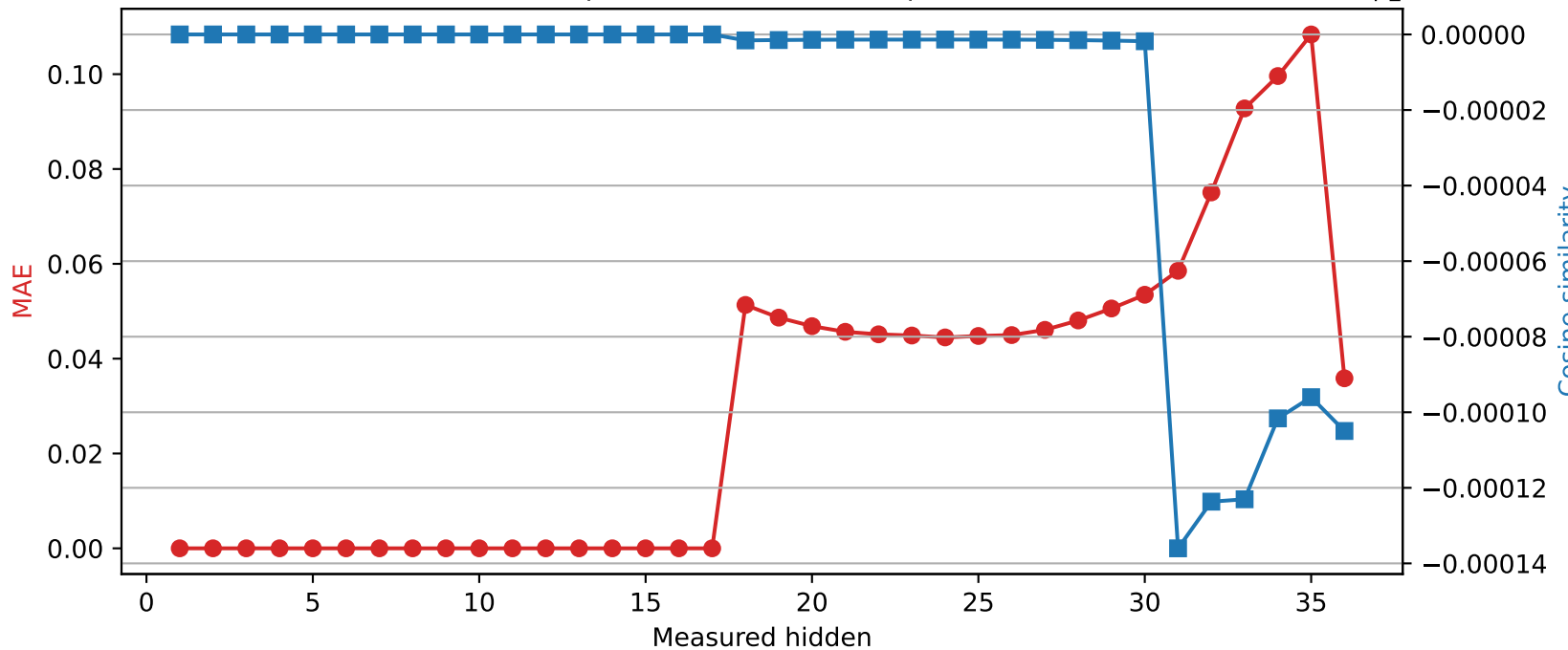
Qwen2.5-3B | Quantized layer 17 | float64 → int8
