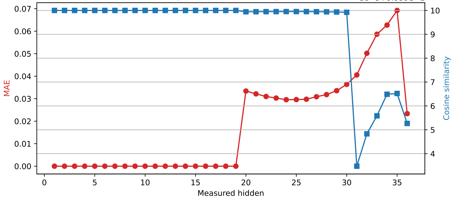
Qwen2.5-3B | Quantized layer 19 | float64 → int8
