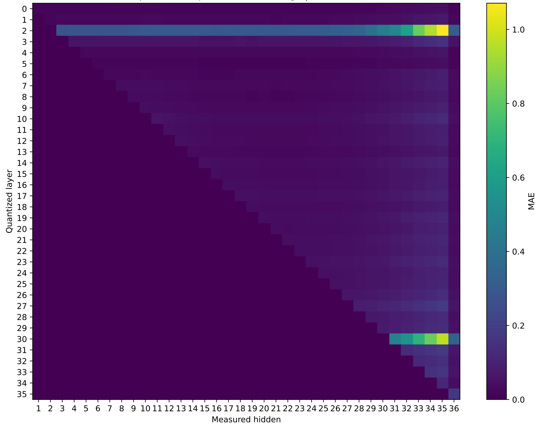
Qwen2.5-3B Prompt 1: MAE representation damage | float64 → int8
