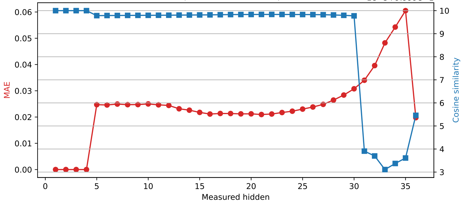
Qwen2.5-3B | Quantized layer 4 | float64 → int8
