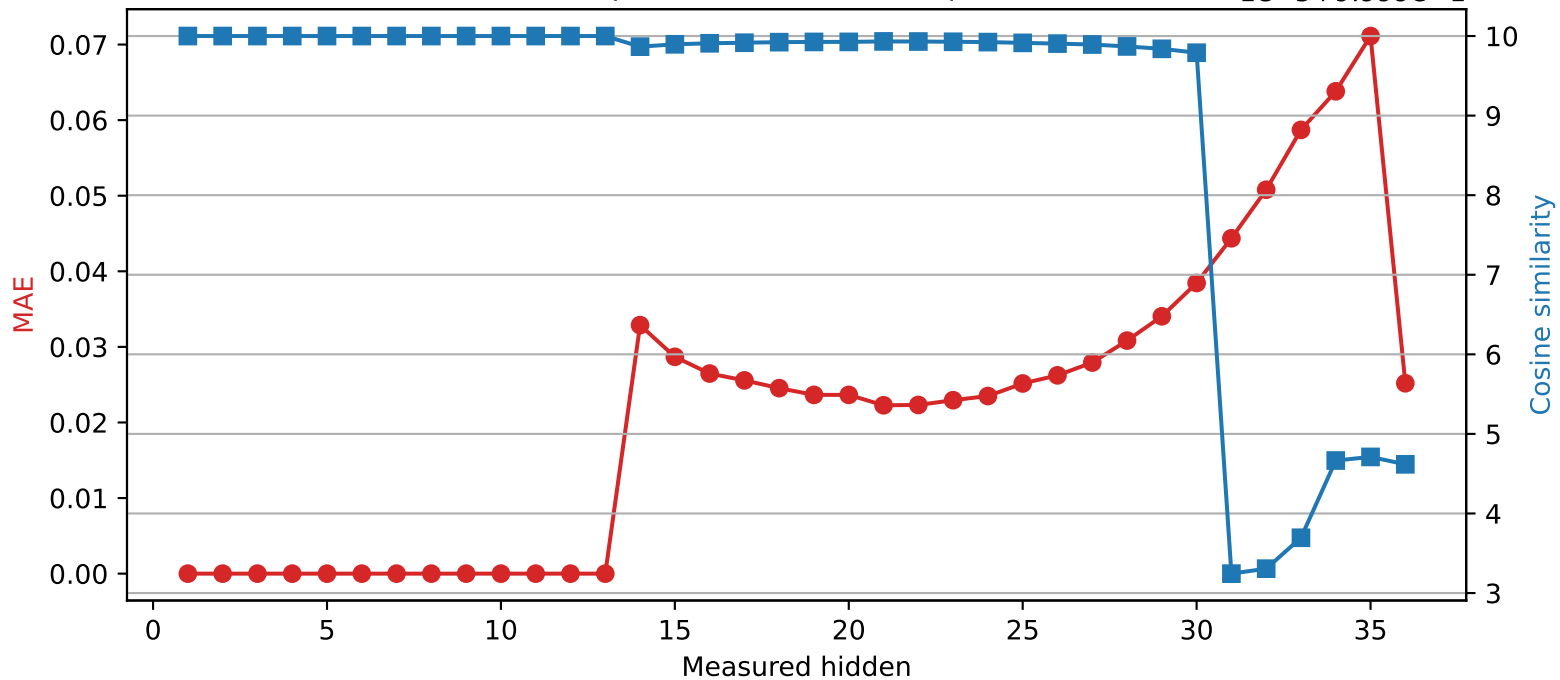
Qwen2.5-3B | Quantized layer 13 | float64 → int8
