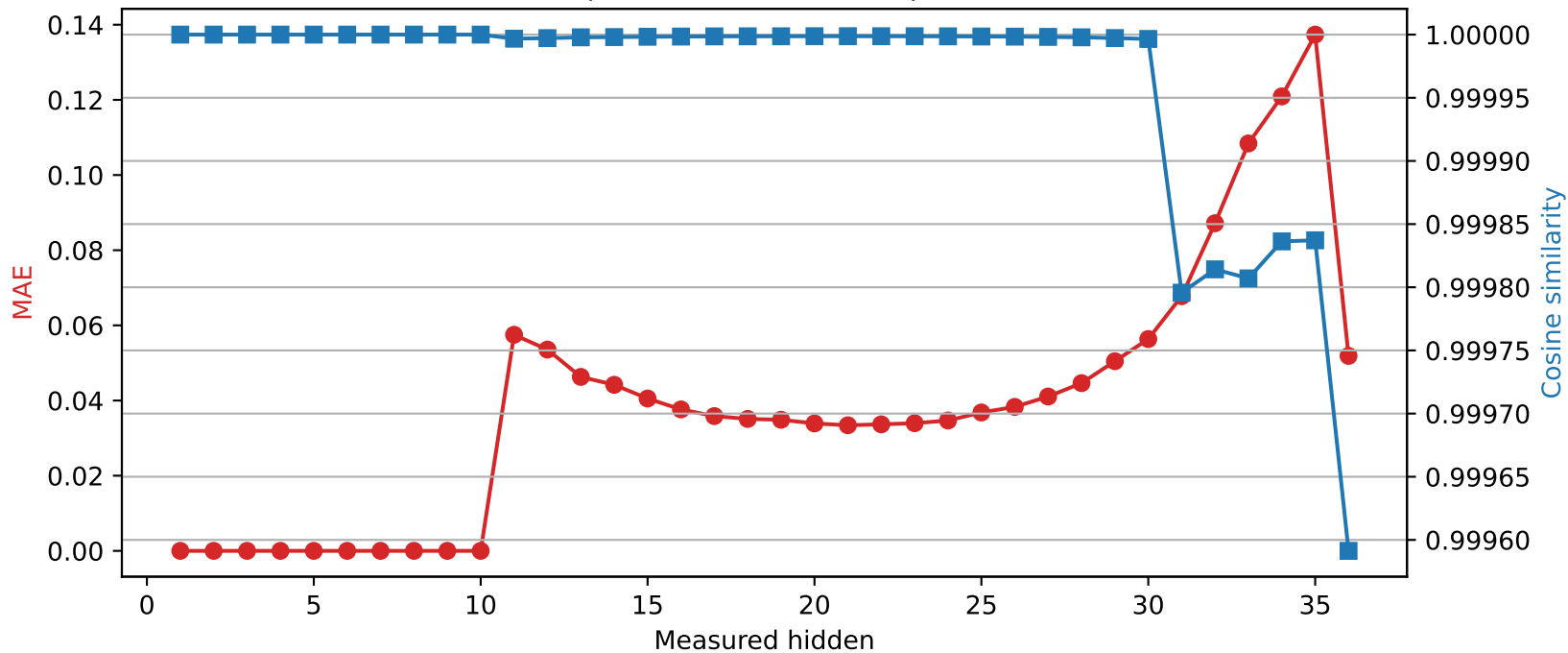
Qwen2.5-3B | Quantized layer 10 | float64 → int8
