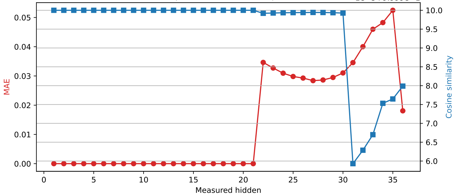
Qwen2.5-3B | Quantized layer 21 | float64 → int8
