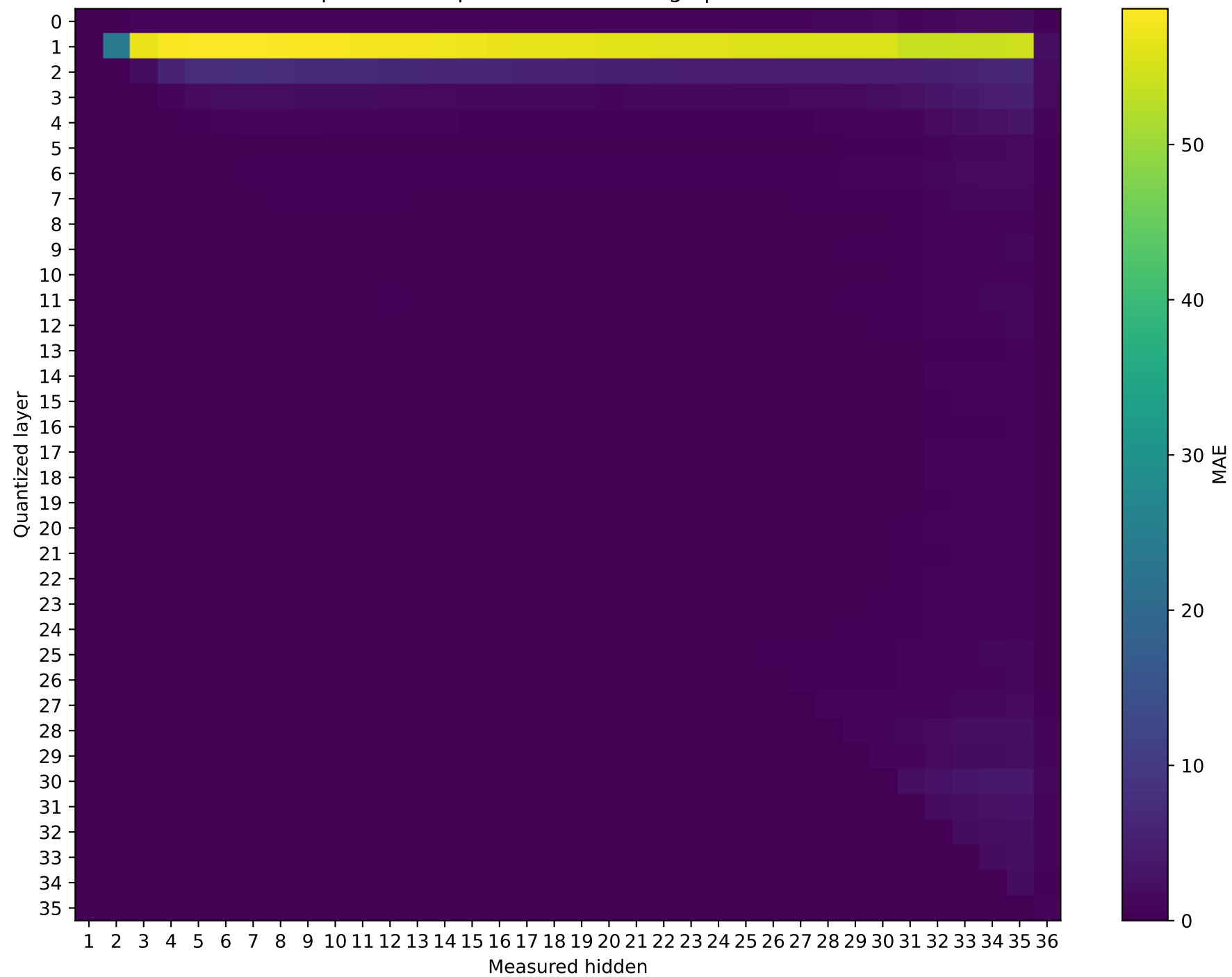
Qwen2.5-3B Prompt 0: MAE representation damage | float16 \rightarrow int4
