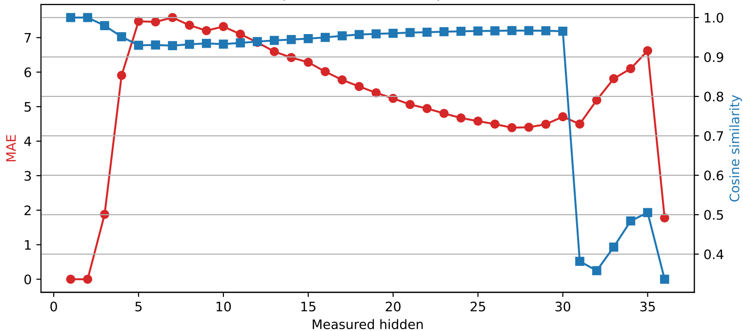
Qwen2.5-3B | Quantized layer 2 | float16 \rightarrow int4
