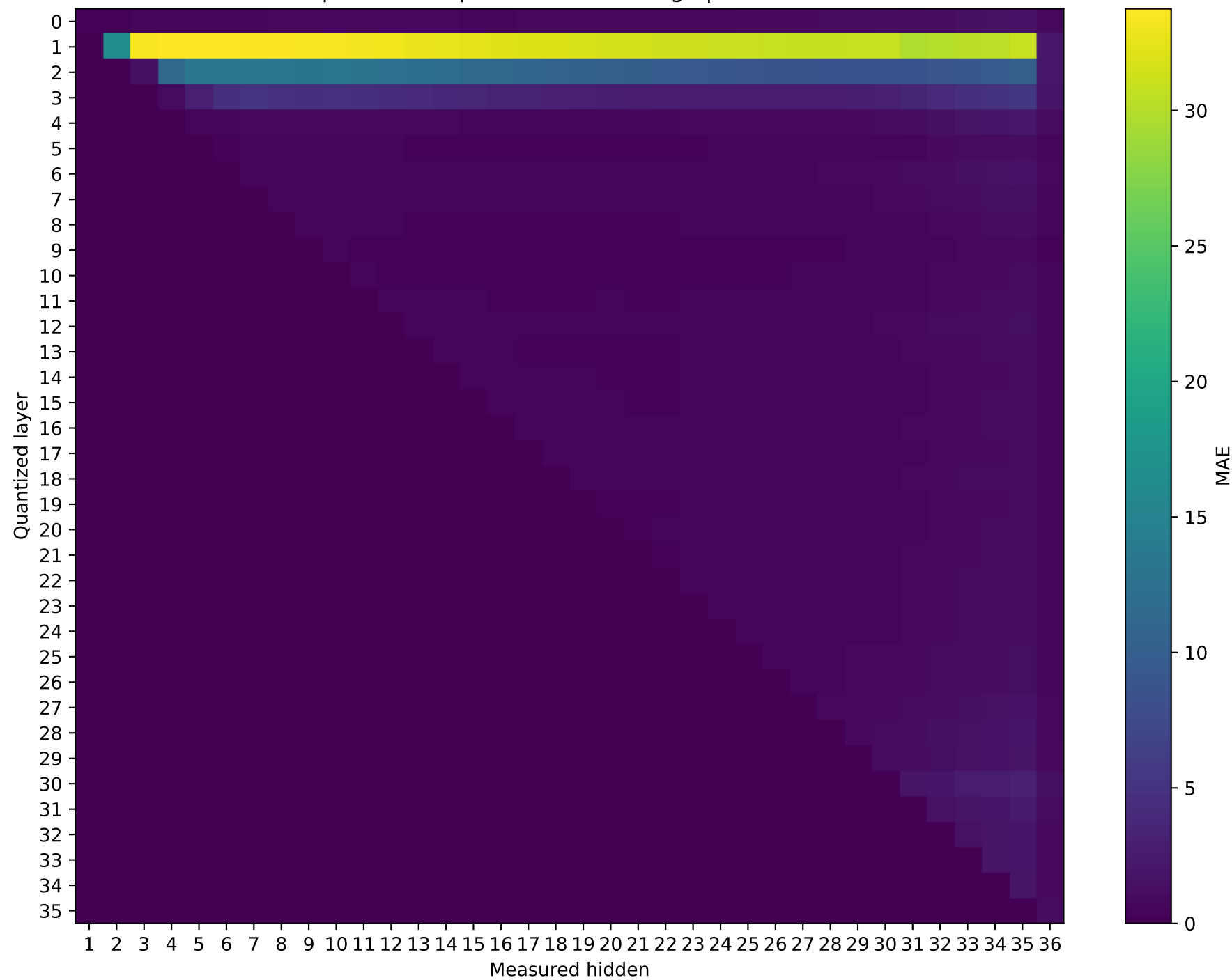
Qwen2.5-3B Prompt 2: MAE representation damage | float16 → int4
