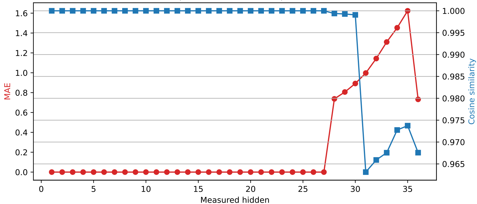
Qwen2.5-3B | Quantized layer 27 | float16 → int4
