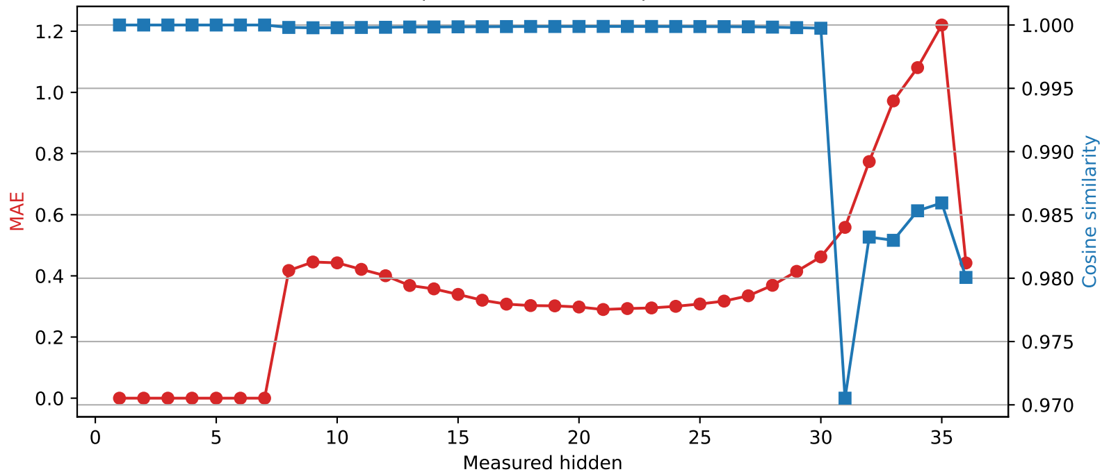
Qwen2.5-3B | Quantized layer 7 | float16 \rightarrow int4
