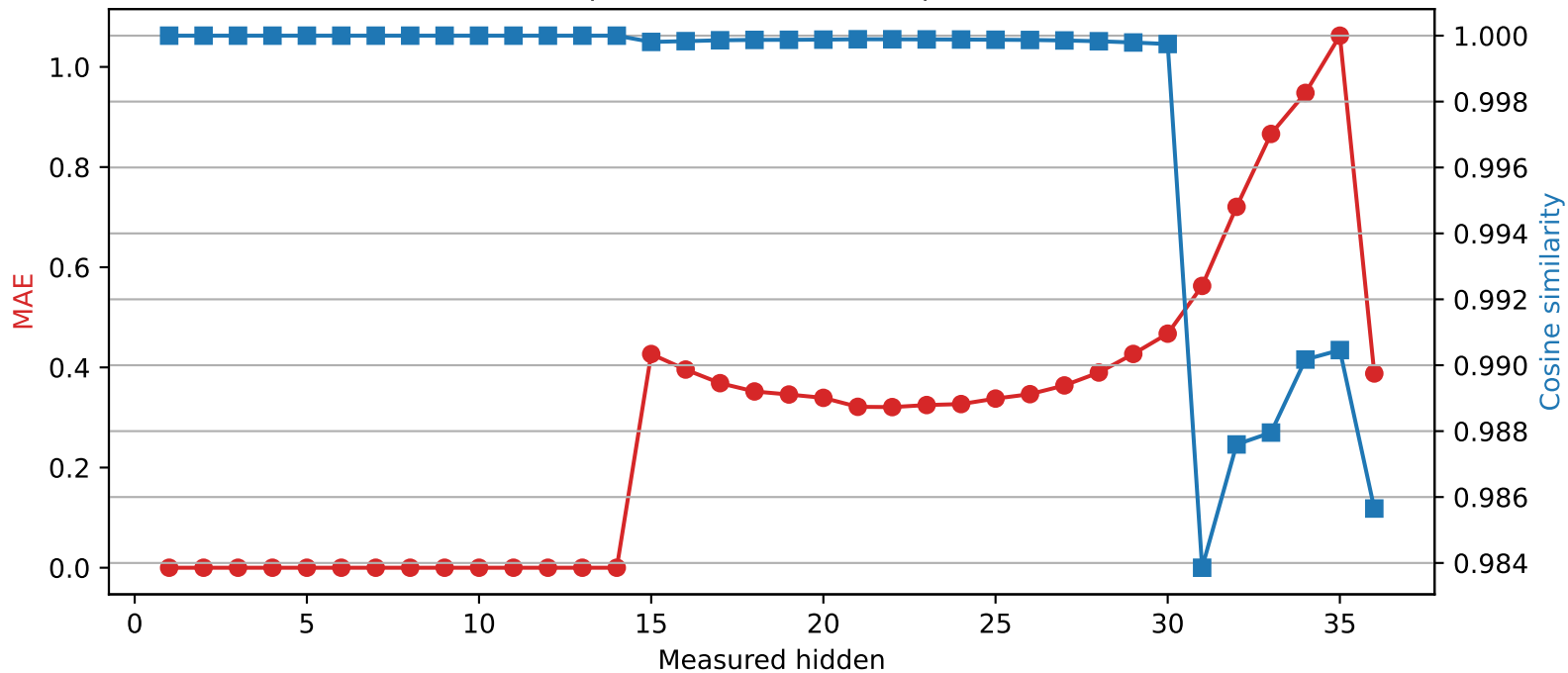
Qwen2.5-3B | Quantized layer 14 | float16 → int4
