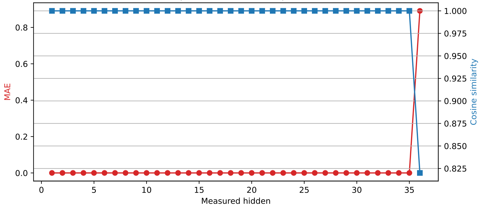
Qwen2.5-3B | Quantized layer 35 | float16 → int4
