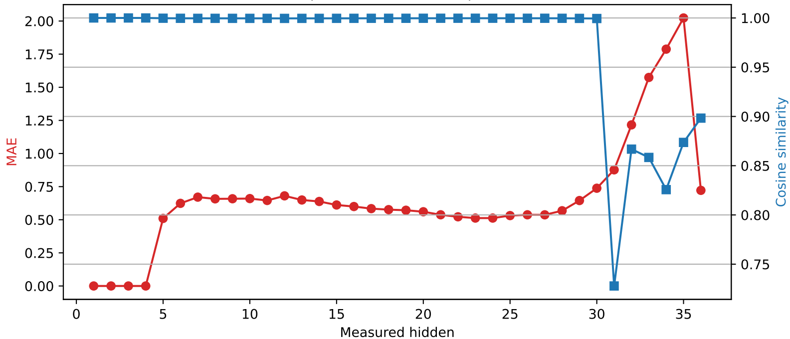
Qwen2.5-3B | Quantized layer 4 | float16 → int4
