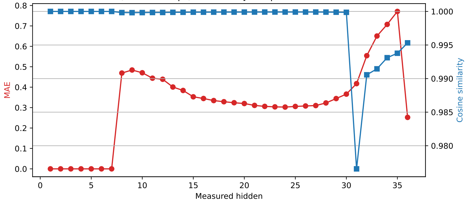
Qwen2.5-3B | Quantized layer 7 | float16 → int4
