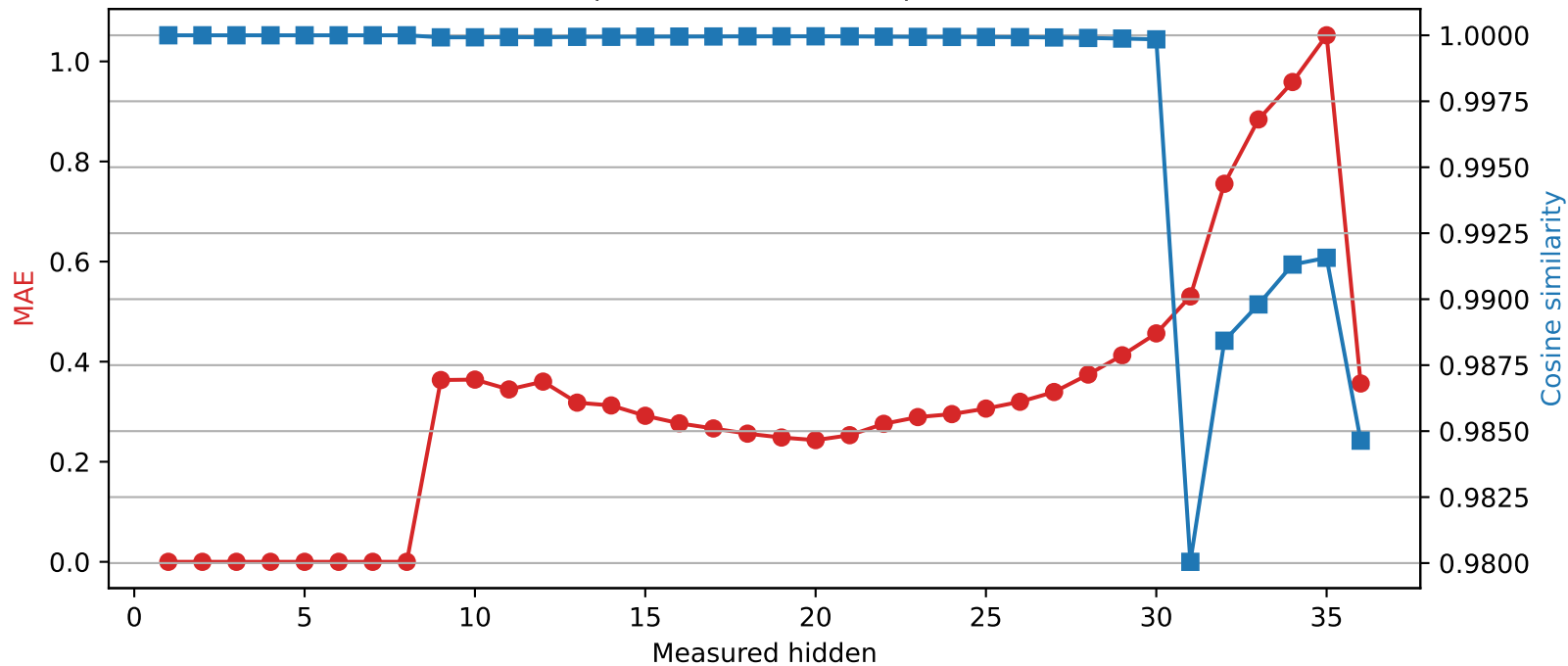
Qwen2.5-3B | Quantized layer 8 | float32 → int4
