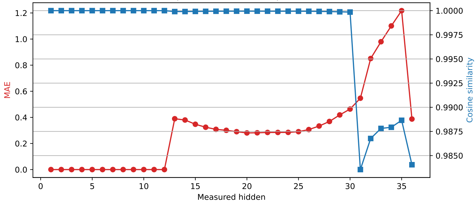
Qwen2.5-3B | Quantized layer 12 | float32 → int4
