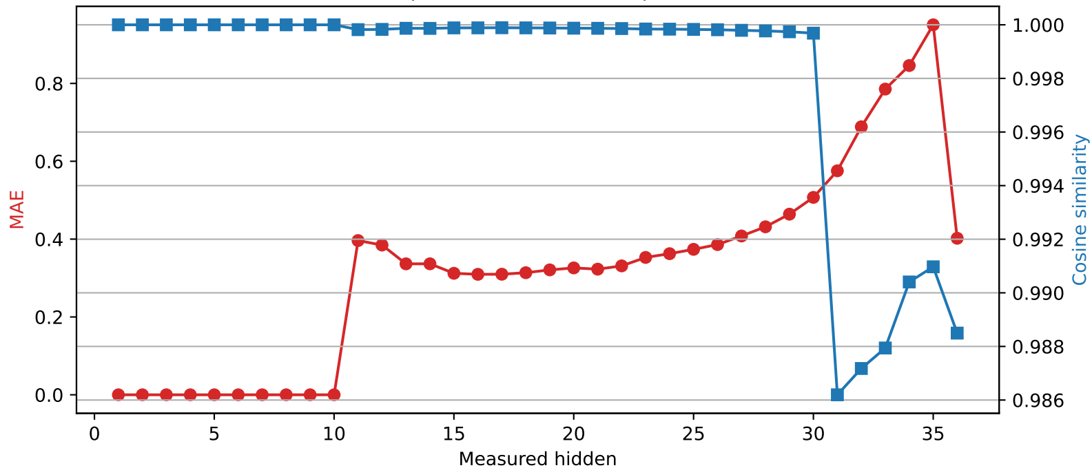
Qwen2.5-3B | Quantized layer 10 | float32 → int4
