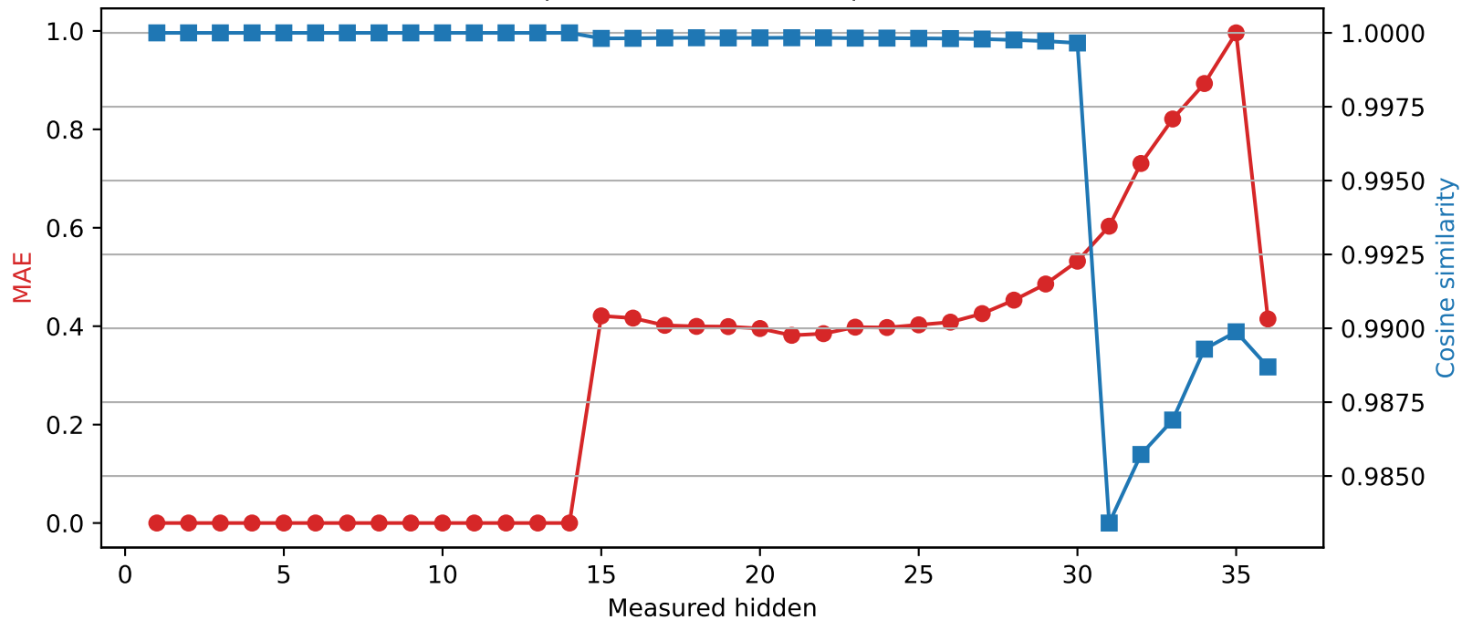
Qwen2.5-3B | Quantized layer 14 | float32 → int4
