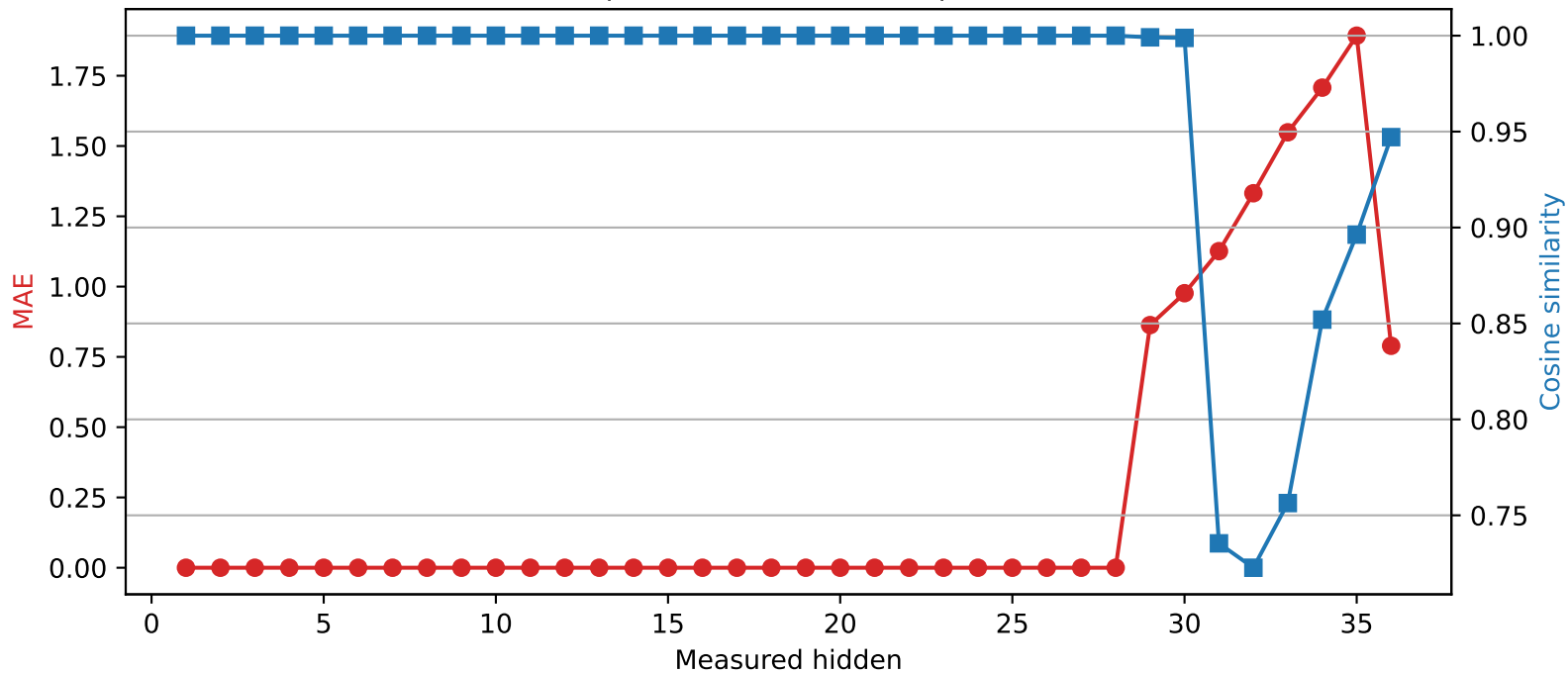
Qwen2.5-3B | Quantized layer 28 | float32 → int4
