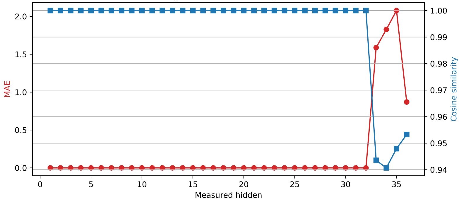
Qwen2.5-3B | Quantized layer 32 | float32 → int4
