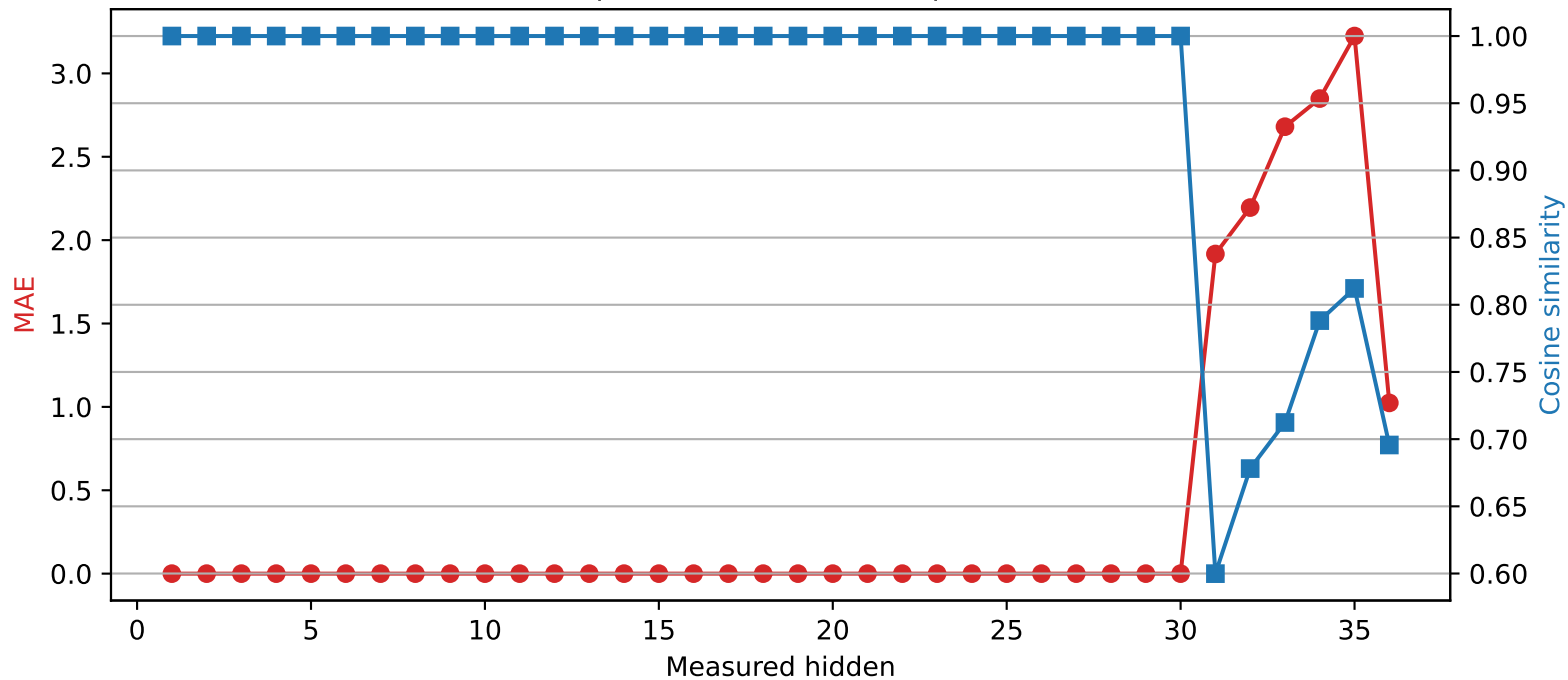
Qwen2.5-3B | Quantized layer 30 | float32 → int4
