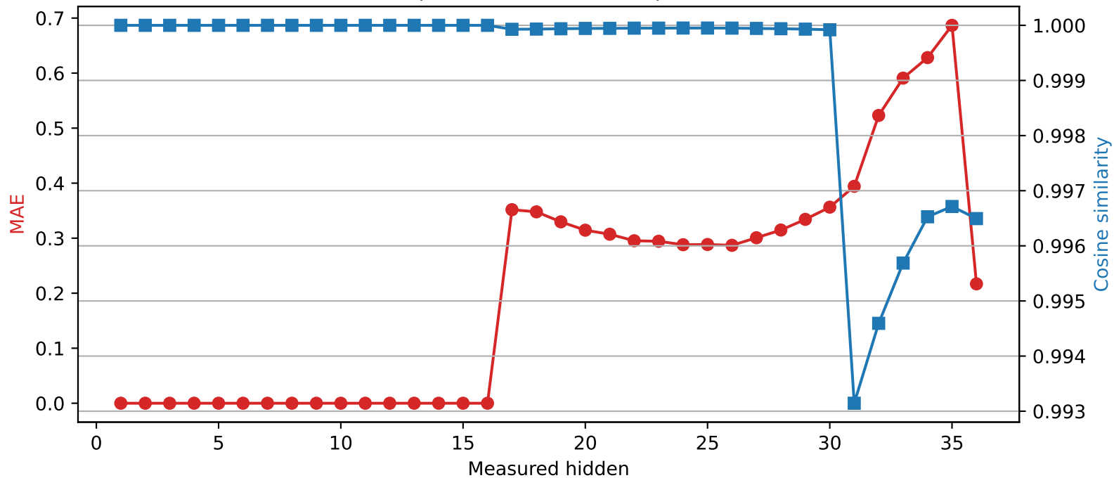
Qwen2.5-3B | Quantized layer 16 | float64 → int4
