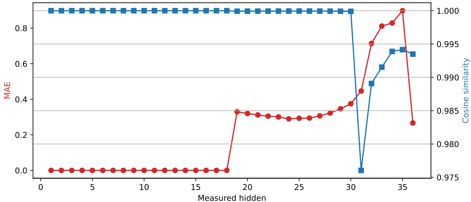
Qwen2.5-3B | Quantized layer 18 | float64 → int4
