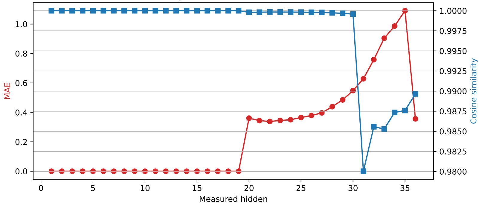
Qwen2.5-3B | Quantized layer 19 | float64 → int4
