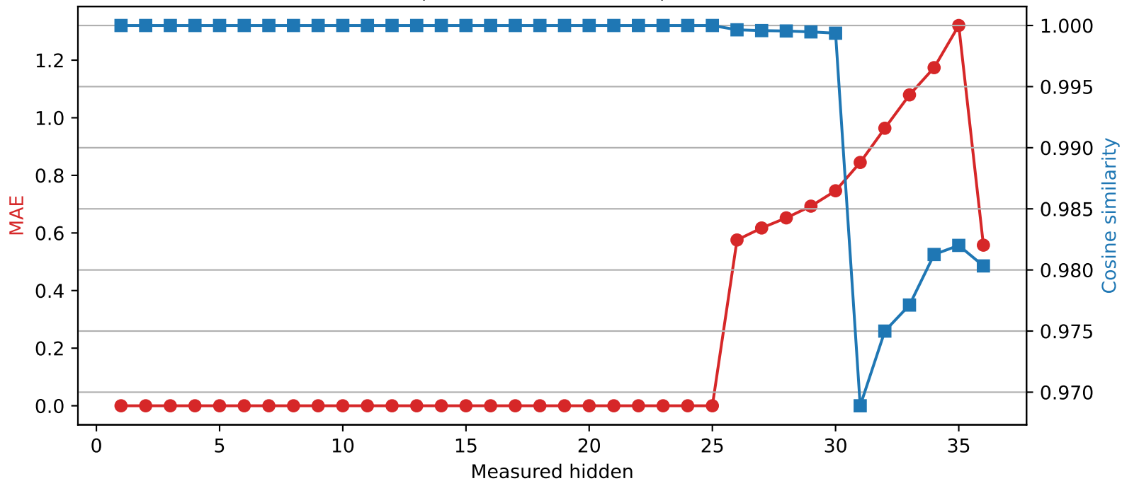
Qwen2.5-3B | Quantized layer 25 | float64 → int4
