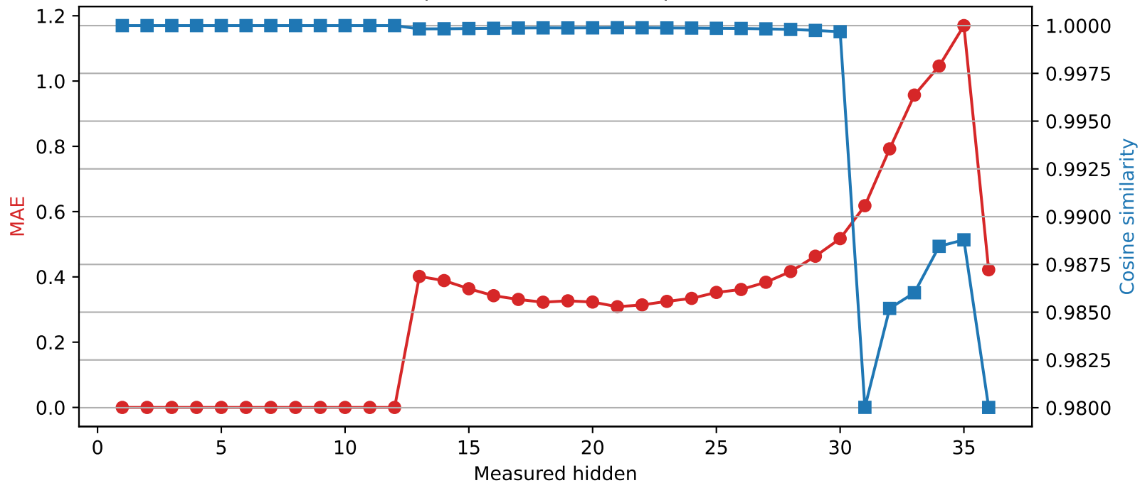
Qwen2.5-3B | Quantized layer 12 | float64 → int4
