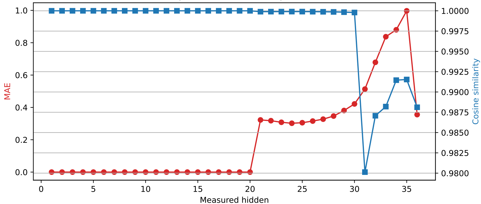
Qwen2.5-3B | Quantized layer 20 | float64 → int4
