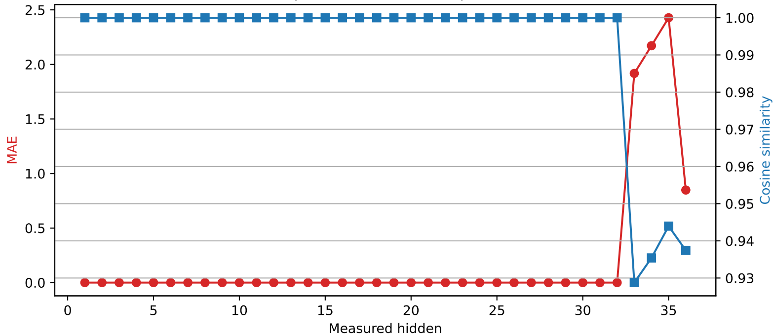
Qwen2.5-3B | Quantized layer 32 | float64 → int4
