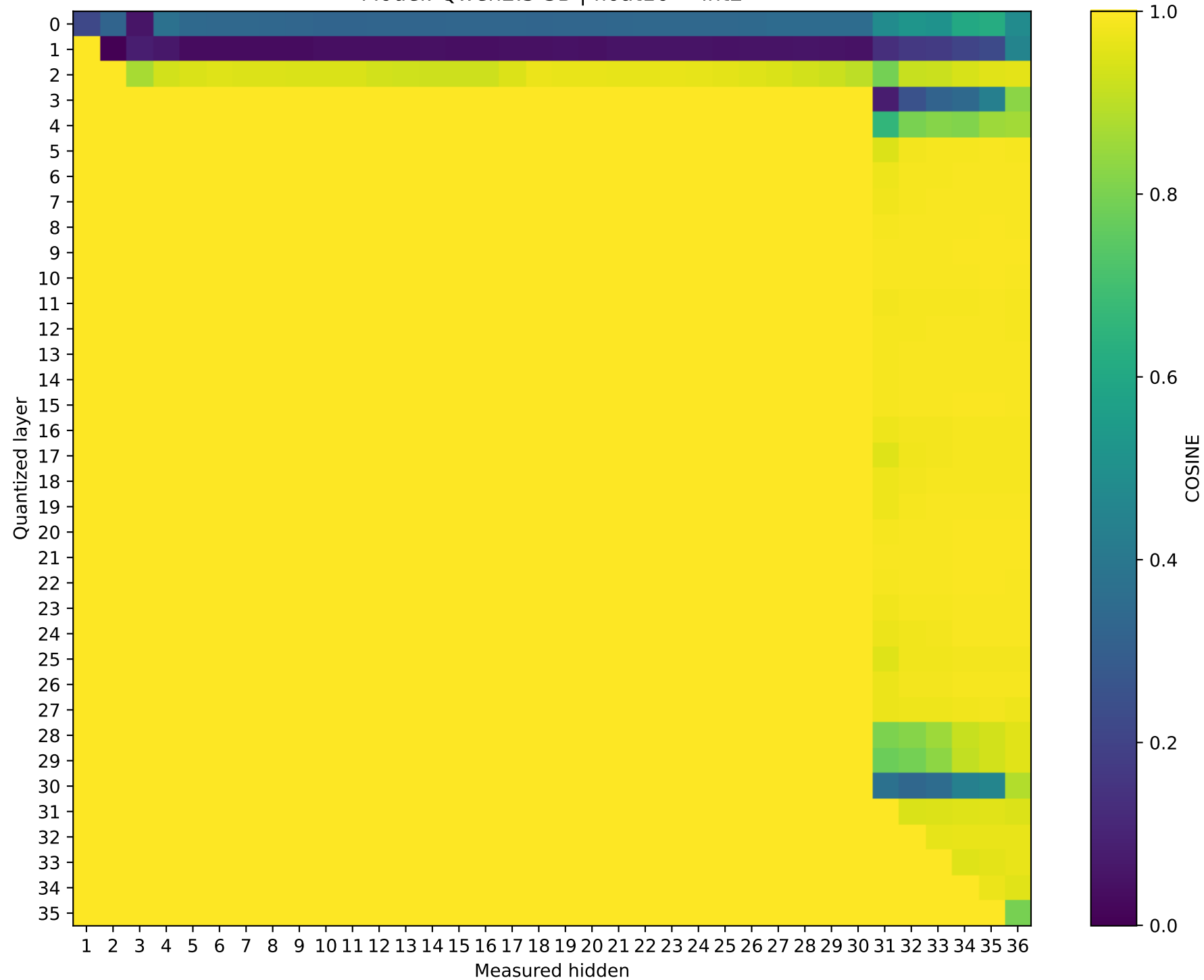
Model: Qwen2.5-3B | float16 \rightarrow int2
